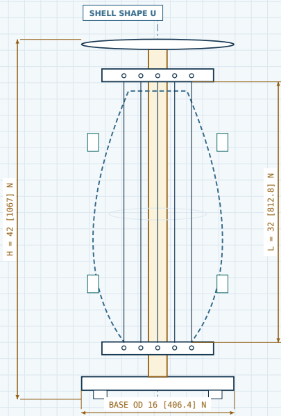
01 / FRONT ELEVATION
