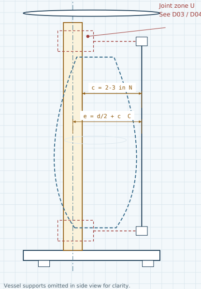
02 / SIDE ELEVATION (+y TO RIGHT)
